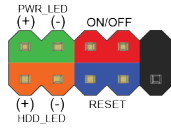
Figure : Front Panel Connector(J_FIO_1)
