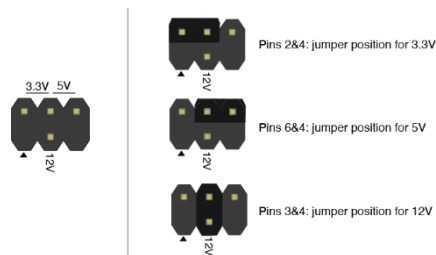
Figure : Panel power Header pin-out(J20)
