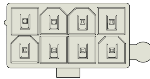
Figure: ATX 8pin pin-out(ATX8P_1)
