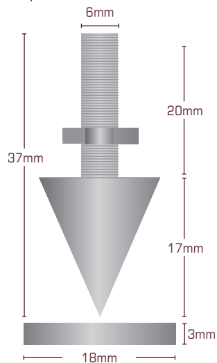
Spike with nut
